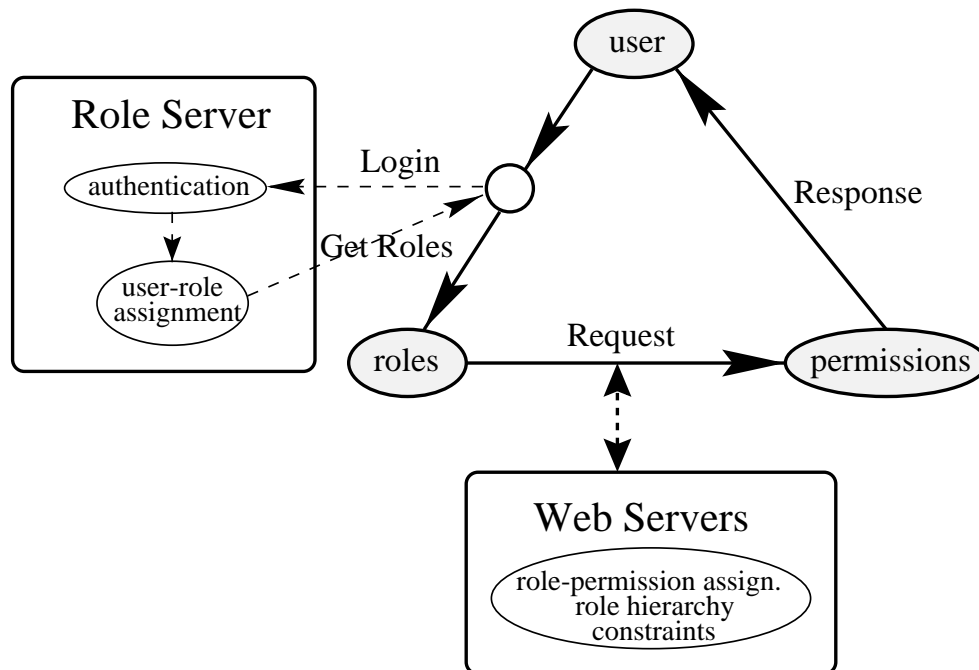
Figure 1: A Schematic of RBAC on the Web
