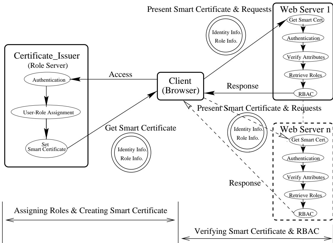
Figure 2: RBAC on the Web by Smart Certificate
