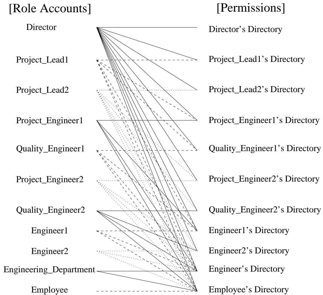
Figure 4: Permission-Account Assignment (PAA)
