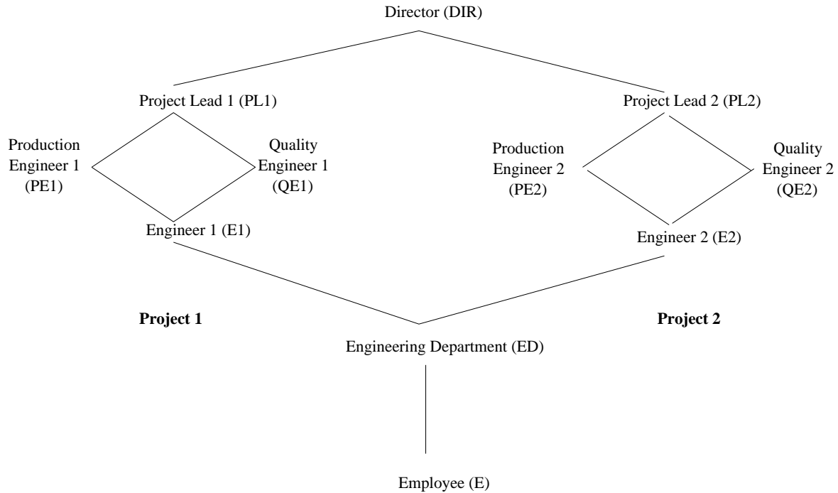
Figure 3: An Example Role Hierarchy
