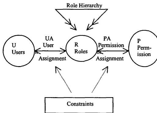
Figure 1: Simplified Version of RBAC96 Model
