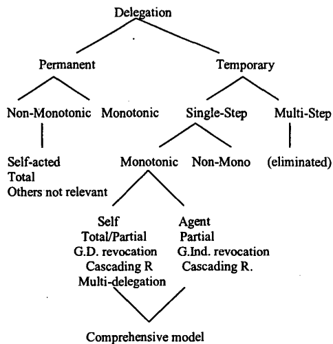
Figure2: Tree structure showing the partitioning process
